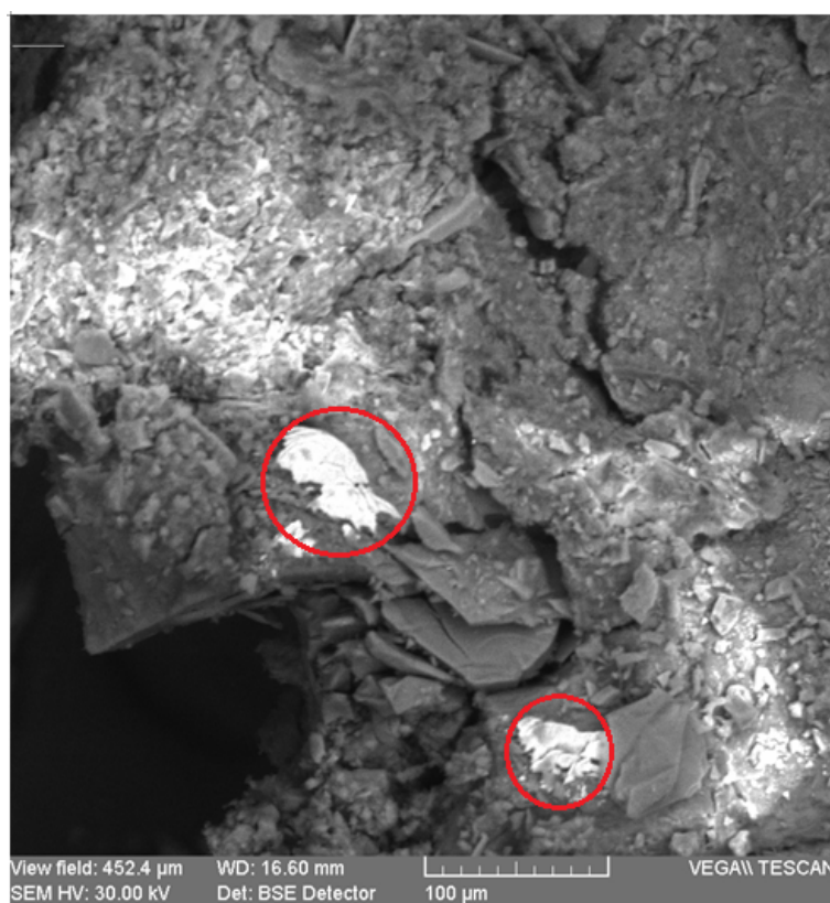
Fig. 2. SEM image of sample no. 6 at 500X magnification. Contamination with an object containing Fe, Cr, C
