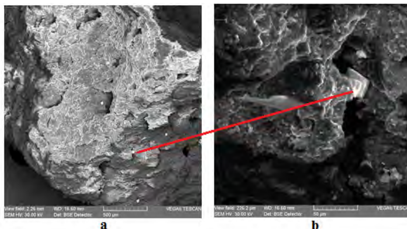
Fig. 1. SEM images of sample no. 6: inclusion with Sulph and Barium a – overall image, with 100X magnification of its interior, b – inclusion detail on a 1000X magnification
